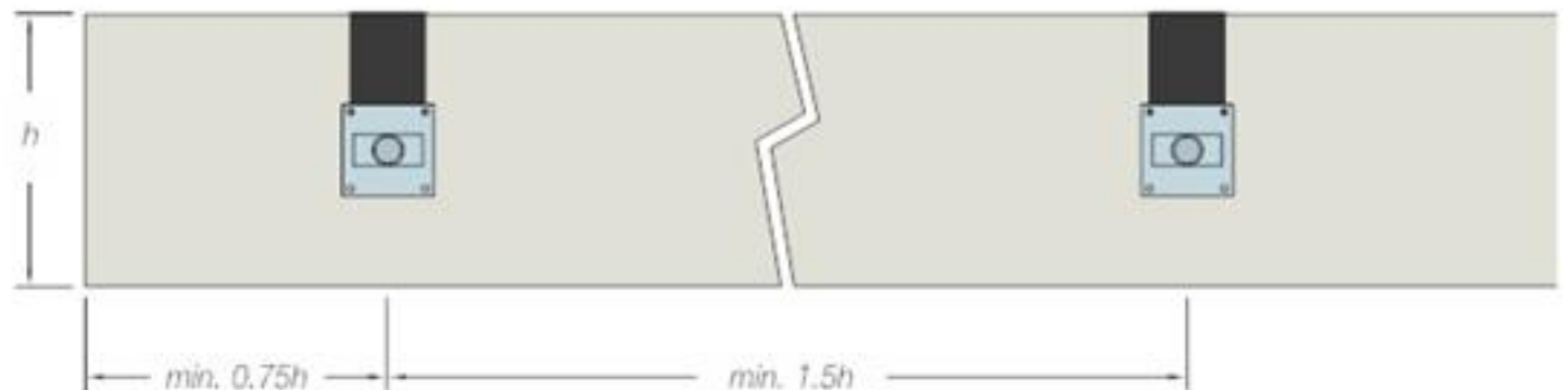
ESDQ-L20 Minimum Edge Distance and Spacings
