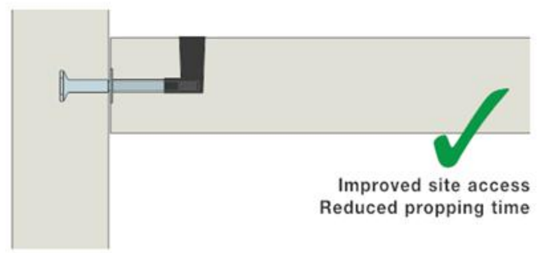
Ancon Lockable Dowel
