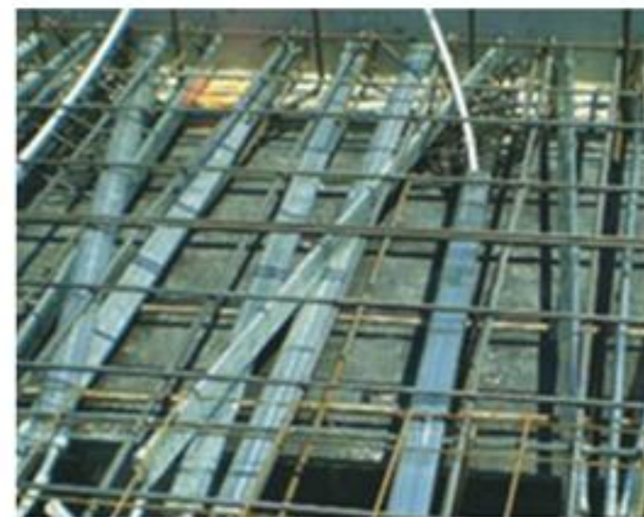
The performance of site assembled systems can be unreliable
