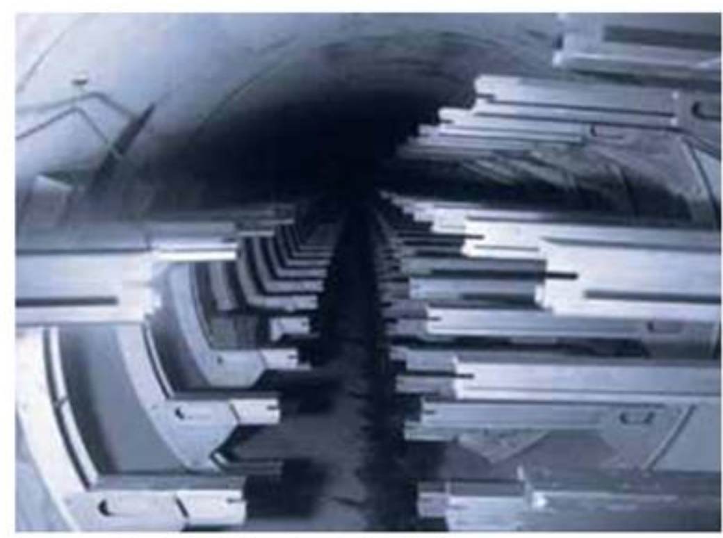
Project: Carlton Cable Tunnel, Australia (Client: Energy Australia, Contractor: The Abergeldie Group, Cable Support Engineering: Ancon)
