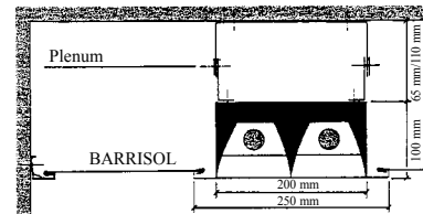
Installation (sectional view)
