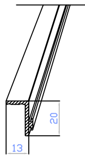
BS 355/30 complement to BS 355/25
