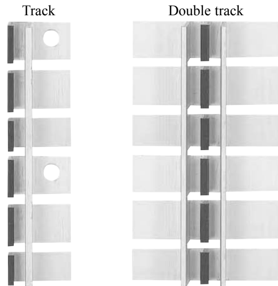
Tracks pre-notched in the factory to adapt to curved lines exactly
