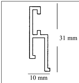
BS 350/01 To be fixed to wall
