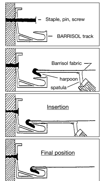
Sectional view of installation
