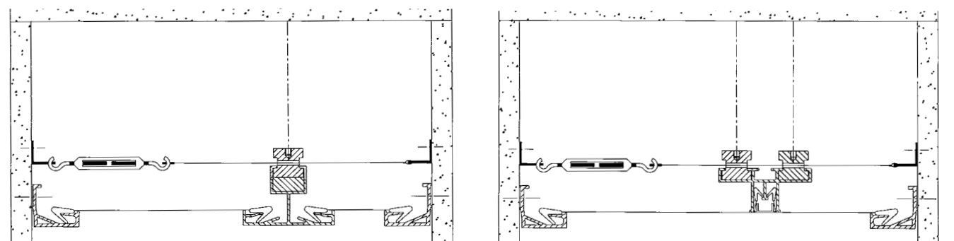
Very high plenum height: the separator is fixed at regular intervals to the ceiling with steel cables and to the wall with stretching devices.
