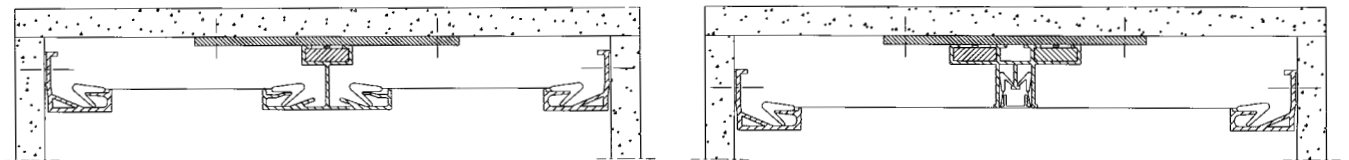
Low plenum height: the separator is fixed to the ceiling
