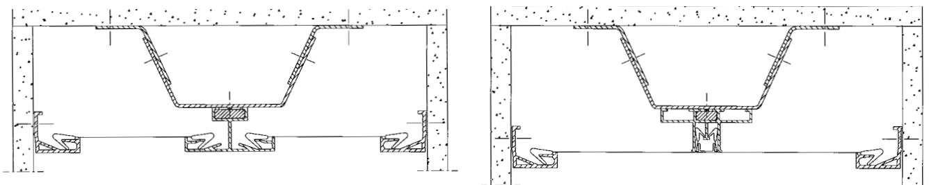
High plenum height: the separator is fixed to the ceiling, at regular intervals, with an adjustable device.
