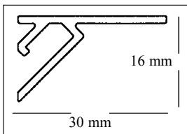
BS 350/202 To be fixed to ceiling
