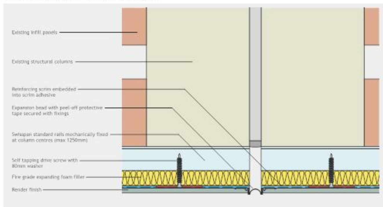
Swisspan expansion joint detail (plan)
