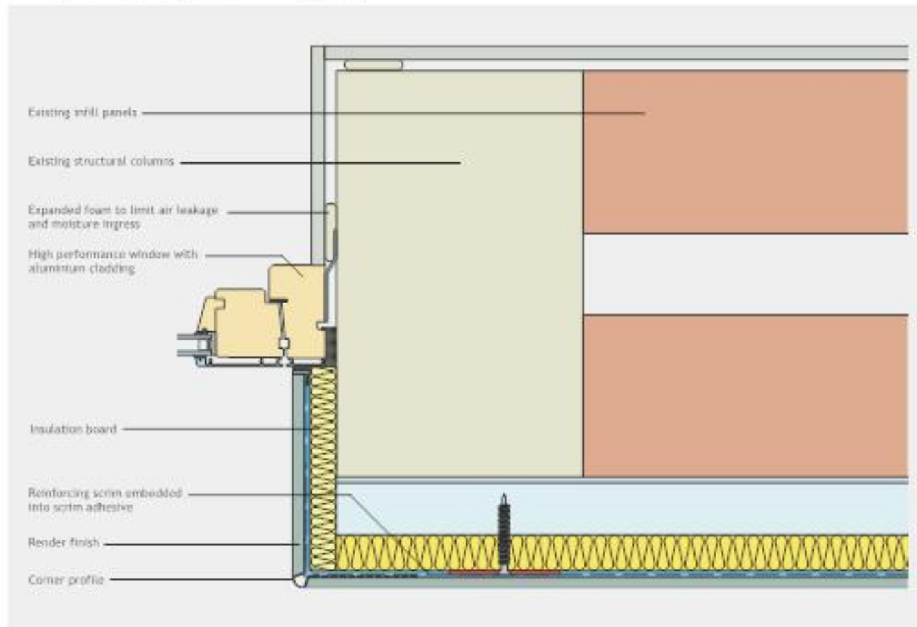
Swisspan window jamb detail (plan)
