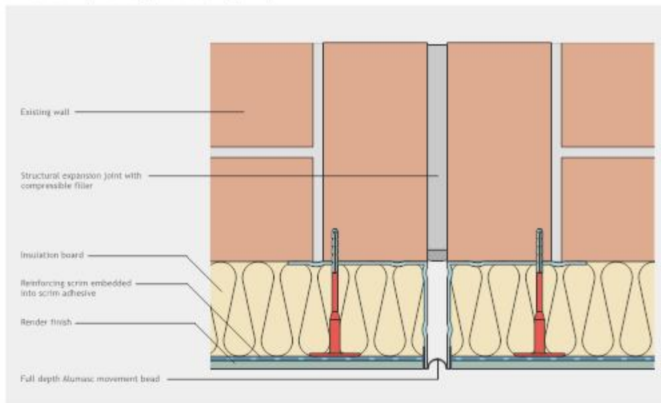
Swisslab expansion joint detail (plan)
