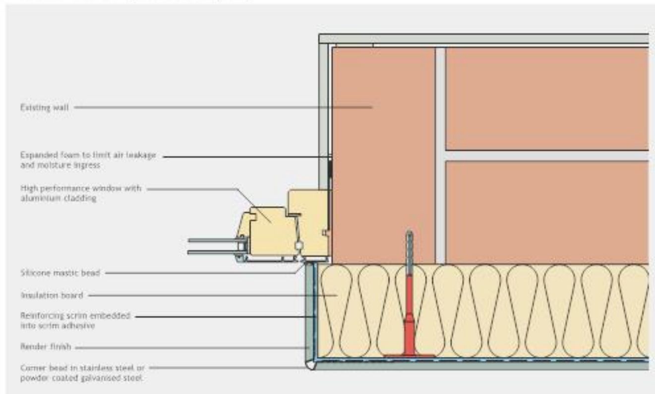
Swisslab window jamb detail (plan)
